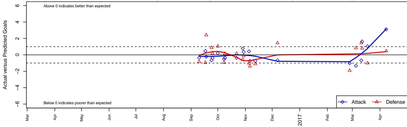
Crossfire OR WUSC Navy G04 Dots are actual minus expected GF (blue circles) and GA (red triangles). Blue line is smoothed change in attack strength. Red is smoothed change in defense strength.
